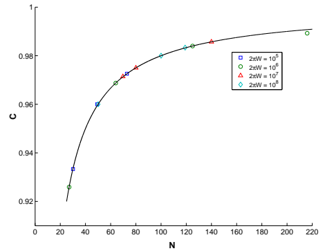
FIG. 4: Behavior of C(N) in the Dicke limit.
