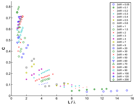
FIG. 2: Behavior of C as a function of the size a = L/\lambda \geq 1 , for different disorder strengths W .
