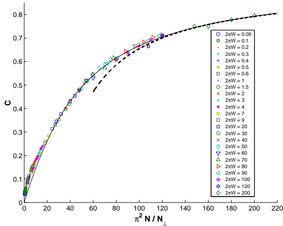
FIG. 3: All points represented in Fig.2 collapse on a single curve as expected from (10). The solid line is a fit of (14) and the dashed line is the asymptotic behavior obtained from (12).
