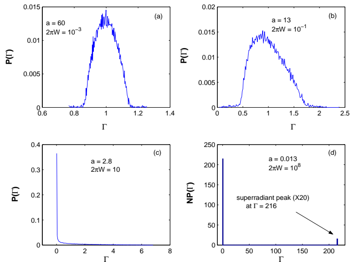
FIG. 1: Behavior of P(\Gamma) for different values of disorder W and size a = L/\lambda , with N = 216 . (a) low disorder (b), (c) larger disorder and (d) Dicke limit.
